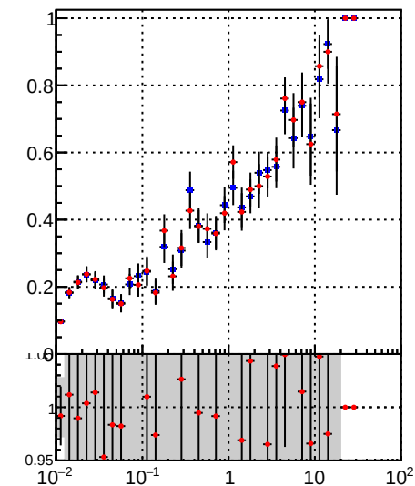
Legend: - Blue line with markers: /data2/legianni/BDT-vs-DNN/real-BDT/CMSSW_13_0_0_pre4/src/runrem/DQM_TT_mkFit_ - Red line with markers: DQM_TT_mkFit_
