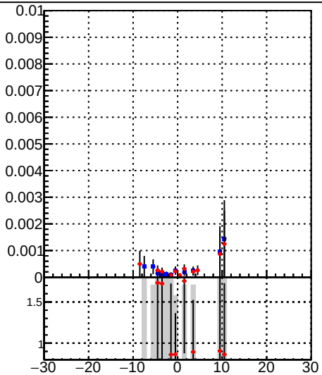
—■— /data2/legianni/BDT-vs-DNN/real-BDT/CMSSW_13_0_0_pre4/src/runrem/DQM_TT_mkFit_ —+— DQM_TT_mkFit_
