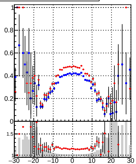
—■— /data2/legianni/BDT-vs-DNN/real-BDT/CMSSW_13_0_0_pre4/src/runrem/DQM_TT_mkFit_ —+— DQM_TT_mkFit_
