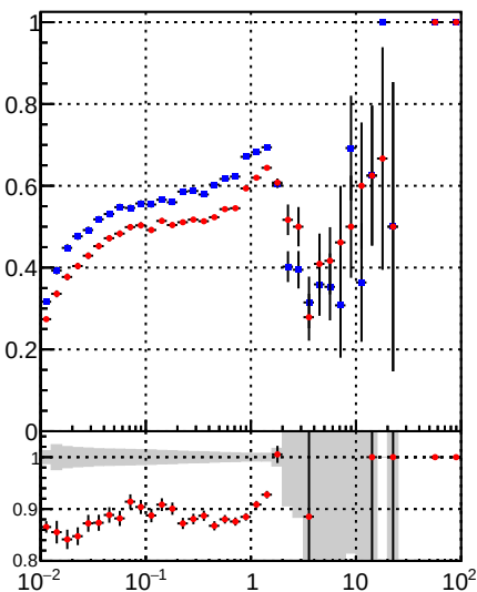
—■— /data2/legianni/BDT-vs-DNN/real-BDT/CMSSW_13_0_0_pre4/src/runrem/DQM_TT_mkFit_ —+— DQM_TT_mkFit_
