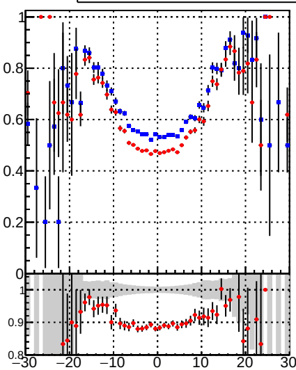
—■— /data2/legianni/BDT-vs-DNN/real-BDT/CMSSW_13_0_0_pre4/src/runrem/DQM_TT_mkFit_ —+— DQM_TT_mkFit_
