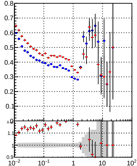
—■— /data2/legianni/BDT-vs-DNN/real-BDT/CMSSW_13_0_0_pre4/src/runrem/DQM_TT_mkFit_ —+— DQM_TT_mkFit_
