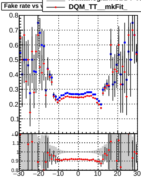
—■— /data2/legianni/BDT-vs-DNN/real-BDT/CMSSW_13_0_0_pre4/src/runrem/DQM_TT_mkFit_ —●— DQM_TT_mkFit_
