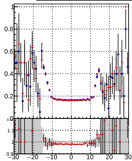
—■— /data2/legianni/BDT-vs-DNN/real-BDT/CMSSW_13_0_0_pre4/src/runrem/DQM_TT_mkFit_ —●— DQM_TT_mkFit_
