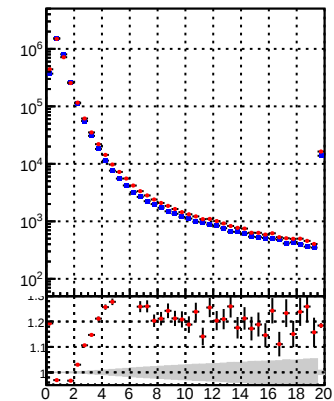
N of reco track vs. \chi^2 for /data2/legianni/BDT-vs-DNN/real-BDT/CMSSW_13_0_0_pre4/src/runrem/DQM_TT_mkFit_ (blue circles) and DQM_TT_mkFit_ (red circles). The grey shaded region indicates the background.
