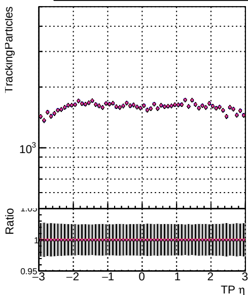
N of sim DOM V0001 R0000000001 Global mkFitNewHpTt RECC DOM V0001 R0000000001 Global mkFitNewDetg RECC DOM V0001 R0000000001 Global mkFitNewDetg RECC
