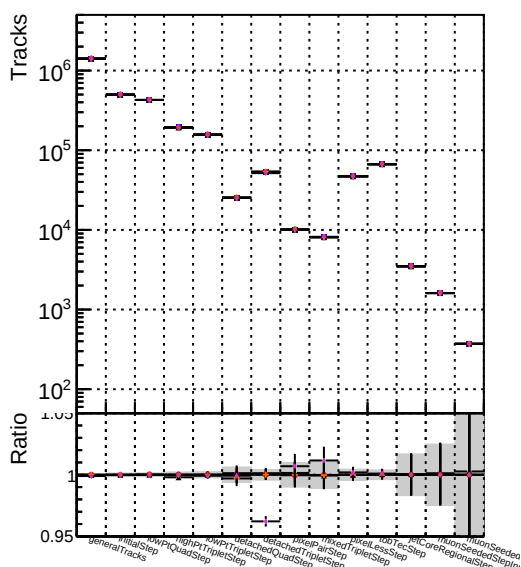
Number Legend DOM V0001 R0000000001 Global mkFitOriginal RECO —●— DOM V0001 R0000000001 Global mkFitNew RECO —●— DOM V0001 R0000000001 Global mkFitNewHpTt RECO —●— DOM V0001 R0000000001 Global mkFitNewDett RECO —●— DOM V0001 R0000000001 Global mkFitNewDett RECO
