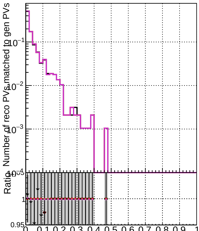
RecoPVAssoc2GenPVmatched_missing
