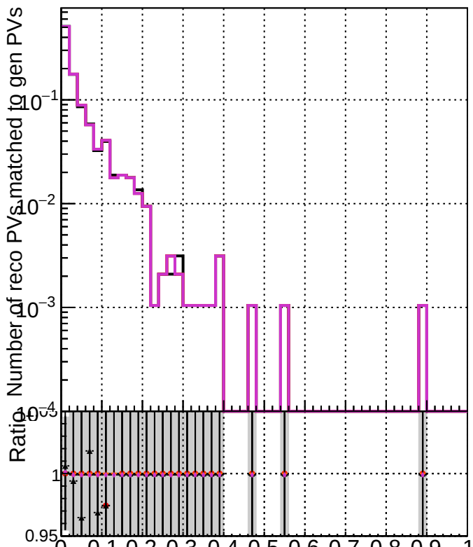
RecoPVAssoc2GenPVmatched_missing
