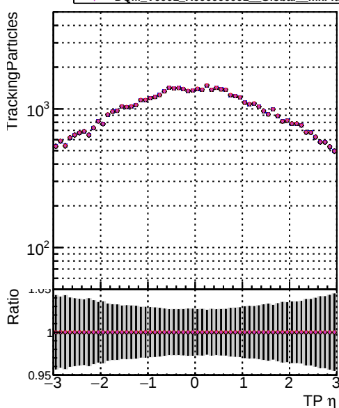
N of sim DOM V0001 R0000000001 Global mkfE Original RECO DOM V0001 R0000000001 Global mkfE New RECO DOM V0001 R0000000001 Global mkfE NewDtt RECO DOM V0001 R0000000001 Global mkfE NewDett RECO DOM V0001 R0000000001 Global mkfE NewDett RECO
