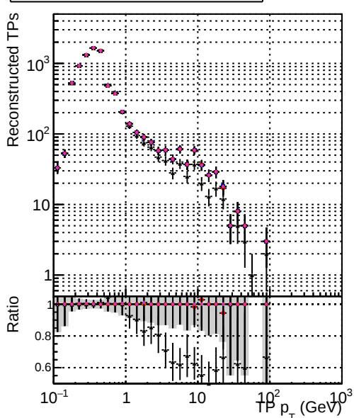
N of sim DOM V0001 R0000000001 Global mkfE Original RECO DOM V0001 R0000000001 Global mkfE New RECO DOM V0001 R0000000001 Global mkfE NewDtt RECO DOM V0001 R0000000001 Global mkfE NewDett RECO DOM V0001 R0000000001 Global mkfE NewDett RECO
