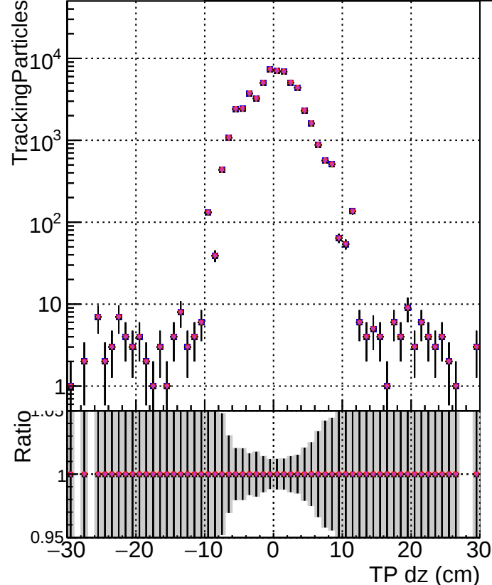
N of simulated track ■ DOM_V0001 R0000000001 Global mkFitOriginal RECO ● DOM_V0001 R0000000001 Global mkFitNew RECO ▲ DOM_V0001 R0000000001 Global mkFitNewHpTt RECO ◆ DOM_V0001 R0000000001 Global mkFitNewDetq RECO ◆ DOM_V0001 R0000000001 Global mkFitNewDett RECO
