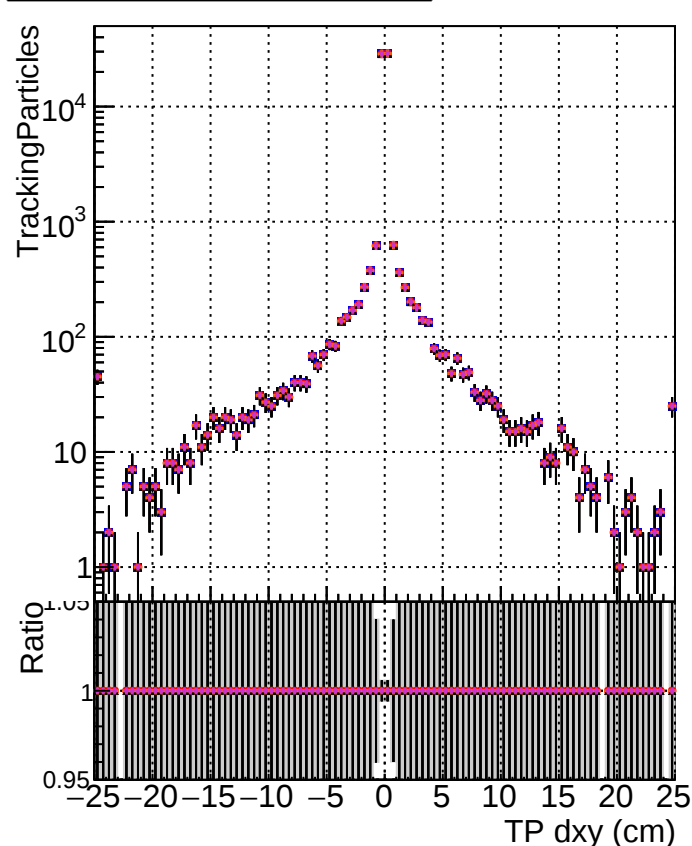
N of simulated track ■ DOM_V0001 R0000000001 Global mkFitOriginal RECO ● DOM_V0001 R0000000001 Global mkFitNew RECO ▲ DOM_V0001 R0000000001 Global mkFitNewHpTt RECO ◆ DOM_V0001 R0000000001 Global mkFitNewDetq RECO ◆ DOM_V0001 R0000000001 Global mkFitNewDett RECO
