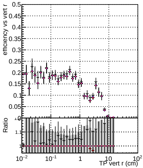
Efficiency DOM V0001 R0000000001 Global mkFitOriginal RECO Blue DOM V0001 R0000000001 Global mkFitOriginal RECO Red DOM V0001 R0000000001 Global mkFitNew RECO Green DOM V0001 R0000000001 Global mkFitNewHPT1 RECO Purple DOM V0001 R0000000001 Global mkFitNewDet1 RECO Black DOM V0001 R0000000001 Global mkFitNewDet1 RECO
