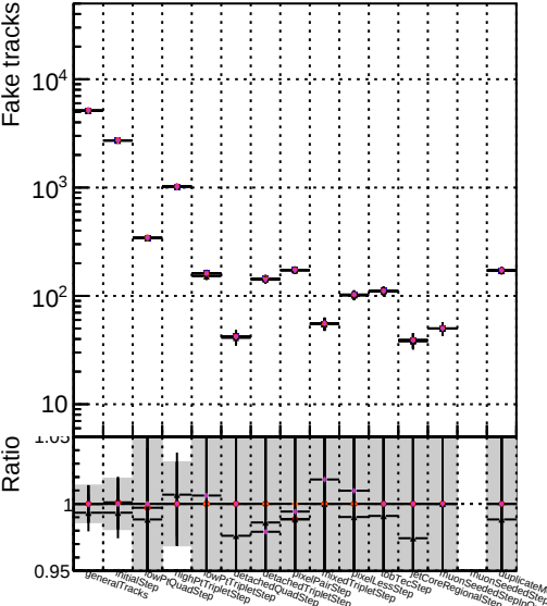
Number DOM V0001 R0000000001 Global mkFit Original RECO DOM V0001 R0000000001 Global mkFit New RECO DOM V0001 R0000000001 Global mkFit NewHpTt RECO DOM V0001 R0000000001 Global mkFit NewDetq RECO DOM V0001 R0000000001 Global mkFit NewDett RECO
