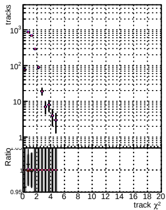
N of reco track vs. \chi^2 for different reconstruction methods
