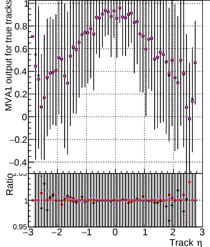
MVA1 of associated tracks (recoToSim) vs. track \eta DOM V0001 R000000001 Global mkFitOriginal RECO DOM V0001 R000000001 Global mkFitNew RECO DOM V0001 R000000001 Global mkFitNewHpTt RECO DOM V0001 R000000001 Global mkFitNewDetg RECO DOM V0001 R000000001 Global mkFitNewDett RECO
