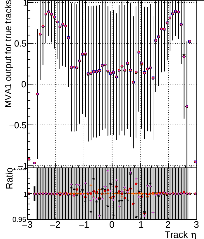
MVA1 of associated tracks (recoToSim) vs. track \eta █ DOM V0001 R0000000001 Global mkFitOriginal RECO ● DOM V0001 R0000000001 Global mkFitNew RECO ▲ DOM V0001 R0000000001 Global mkFitNewHpTt RECO ◆ DOM V0001 R0000000001 Global mkFitNewDetg RECO ◆ DOM V0001 R0000000001 Global mkFitNewDett RECO
