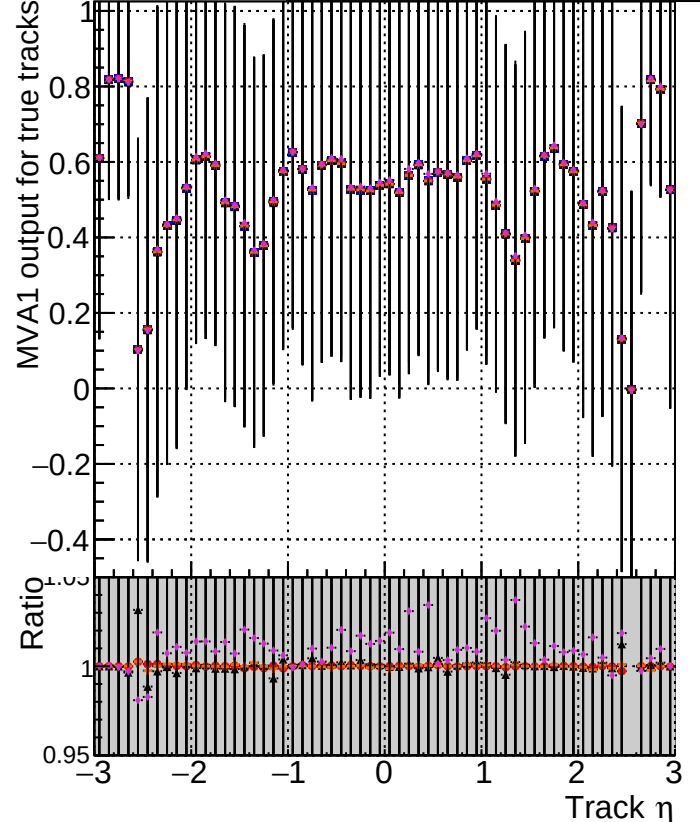
MVA1 of associated tracks (recoToSim) vs. track \eta Legend Model Dataset Fit Type Model Dataset Blue square DOM V0001 R000000001 Global mkFitOriginal RECO Red circle DOM V0001 R000000001 Global mkFitNew RECO Black triangle DOM V0001 R000000001 Global mkFitNewHpTt RECO Orange diamond DOM V0001 R000000001 Global mkFitNewDetg RECO Purple cross DOM V0001 R000000001 Global mkFitNewDett RECO
