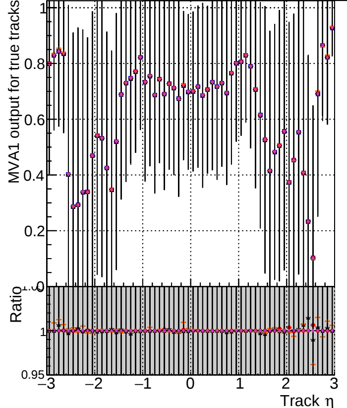
MVA1 of associated tracks (recoToSim) vs. track \eta █ DOM V0001 R000000001 Global mkFitOriginal RECO ● DOM V0001 R000000001 Global mkFitNew RECO ▲ DOM V0001 R000000001 Global mkFitNewHpTt RECO ◆ DOM V0001 R000000001 Global mkFitNewDetg RECO ◆ DOM V0001 R000000001 Global mkFitNewDett RECO
