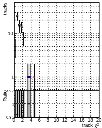
N of reco track vs. \chi^2 for Global fit Original DECO, Global fit NEWBET DECO, and Global fit NEWBET RECO.
