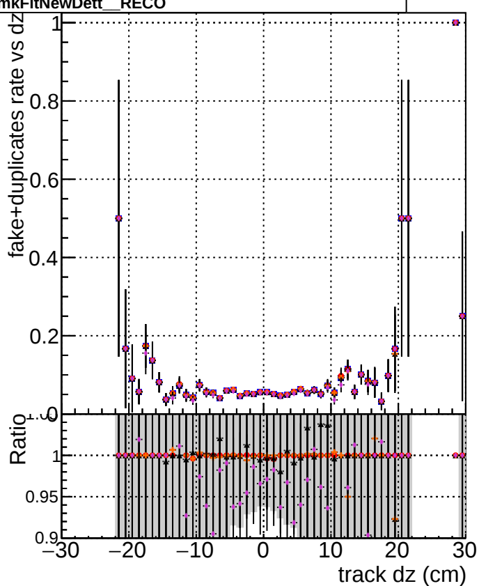
nkFitNewHpTt__RECO
