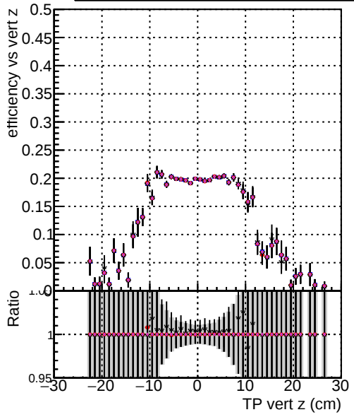
DOM V0001 R0000000001 Global mkFitOriginal RECO DOM V0001 R0000000001 Global mkFitNew RECO DOM V0001 R0000000001 Global mkFitNewHPT1 RECO DOM V0001 R0000000001 Global mkFitNewDetg RECO DOM V0001 R0000000001 Global mkFitNewDetg RECO
