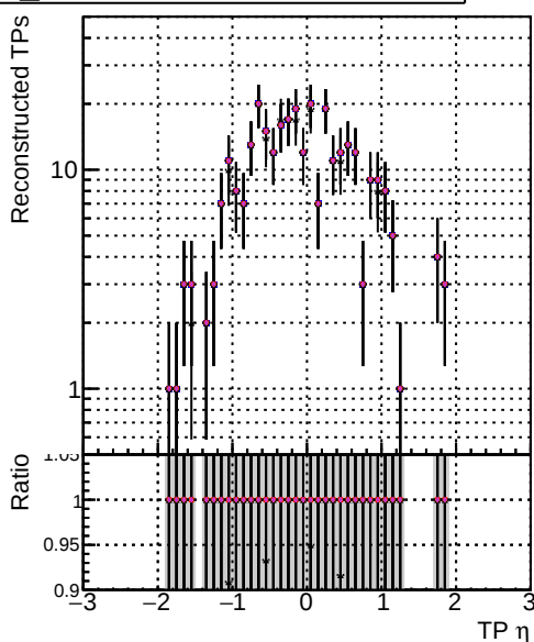
N of Sim DOM V0001 R0000000001 Global mkfE Original RECO DOM V0001 R0000000001 Global mkfE New RECO DOM V0001 R0000000001 Global mkfE NewHPT RECO DOM V0001 R0000000001 Global mkfE NewDeta RECO DOM V0001 R0000000001 Global mkfE NewDett RECO
