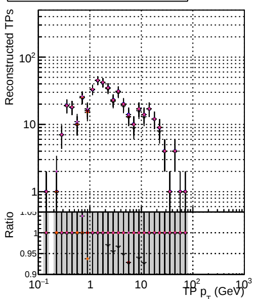
N of Sim DOM V0001 R0000000001 Global mkfE Original RECO DOM V0001 R0000000001 Global mkfE New RECO DOM V0001 R0000000001 Global mkfE NewHPT RECO DOM V0001 R0000000001 Global mkfE NewDeta RECO DOM V0001 R0000000001 Global mkfE NewDett RECO
