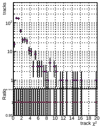
DOM V00001 R0000000000001 Global mkFitOriginal RECO DOM V00001 R0000000000001 Global mkFitNew DetID RECO N of reco track vs. s
