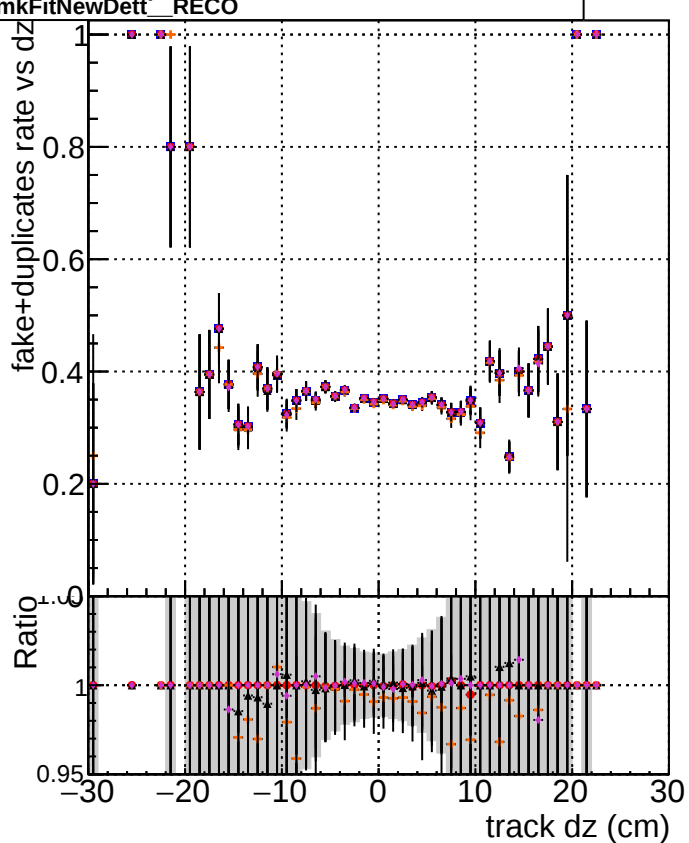
nkFitNewHpTt__RECO
