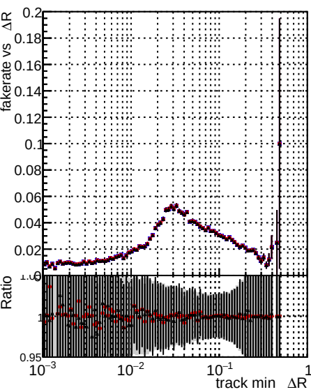
Fake rate vs \Delta R(\text{track, jet}) Legend: - mkFitInItAndFit_CKFHPtT (blue line with dots) - mkFitInItAndFitInnerOuter_CKFHPtT (red line with dots) - mkFitInItAndFitInnerOuter_CKFHPtT_cut4 (black line with dots)
