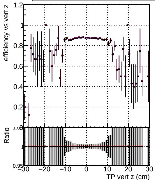
Efficiency vs. TP vert z (cm) mkFitNitAndFit_CKFHPtT mkFitNitAndFitInnerOuter_CKFHPtT mkFitNitAndFitInnerOuter_CKFHPtT_cut4
