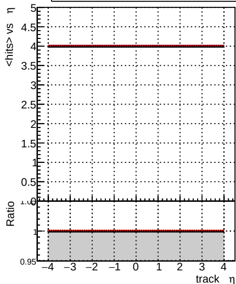
mean hits vs \eta mkFitNitAndFit_CKFHPtT mkFitNitAndFitInnerOuter_CKFHPtT mkFitNitAndFitInnerOuter_CKFHPtT_cut3
