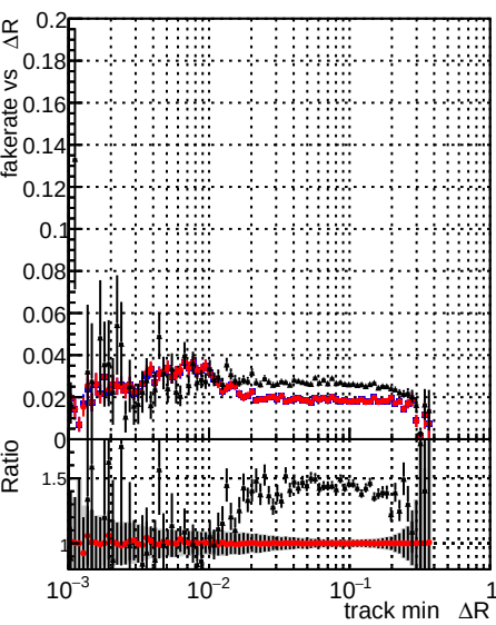
Fake rate vs \Delta R(\text{track, jet}) Legend: - mkFitInitAndFit_CKFHPtT (blue line with dots) - mkFitInitAndFitInnerOuter_CKFHPtT (red line with dots) - mkFitInitAndFitInnerOuter_CKFHPtT_cut3 (black line with dots)
