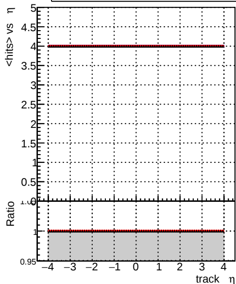
mean hits mkFitNitAndFit_CKFHPtT mkFitNitAndFitInnerOuter_CKFHPtT mkFitNitAndFitInnerOuter_CKFHPtT_cut2
