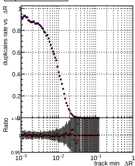
—•— mkFitInitAndFit_CKFHPtT —•— mkFitInitAndFitInnerOuter_CKFHPtT —•— mkFitInitAndFitInnerOuter_CKFHPtT_cut2
