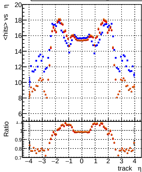
mean hits vs \eta Legend: CKFInit_CKFHPiT (blue line), mkFitInit_CKFHPiT (red line), mkFitInitAndFit_InnerOuter_CKFHPiT (black line), mkFitInitAndFitInnerOuter_CKFHPiT (orange line)
