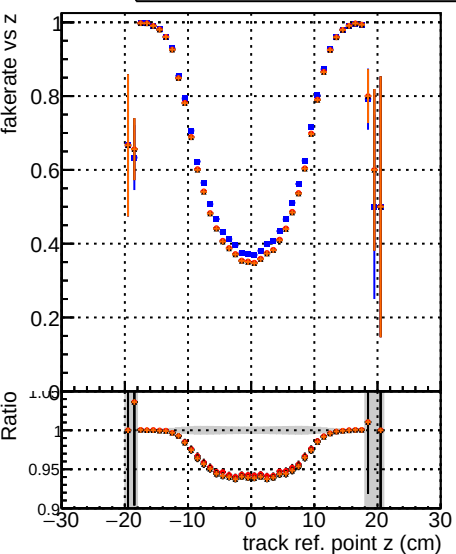
Fake rate vs v CKFHPtT
