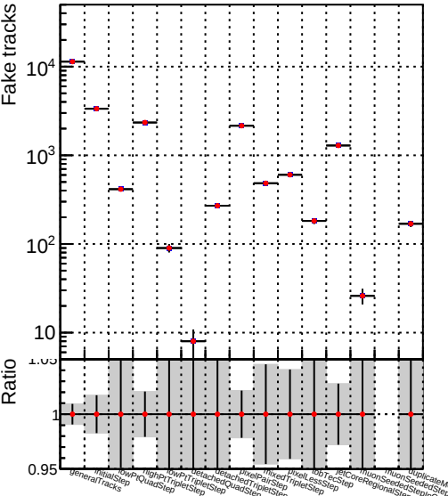
Number —●— DQM_CKF_TTtest125xNEW
