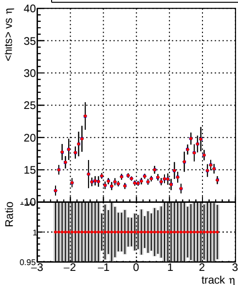
mean hit — DQM_CKF_TTbase — DQM_CKF_TTtest125xNEW
