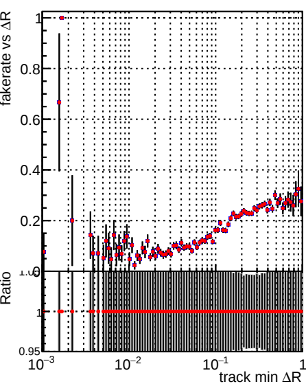
Fake rate vs \Delta R(\text{track, jet}) Legend: \Delta R(\text{track, jet}) (black line with error bars) \Delta R(\text{track, jet}) (red line with error bars)
