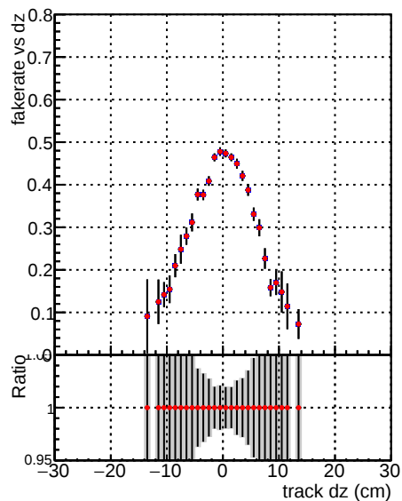
—●— DQM_CKF_TTbase —●— DQM_CKF_TTtest125xNEW
