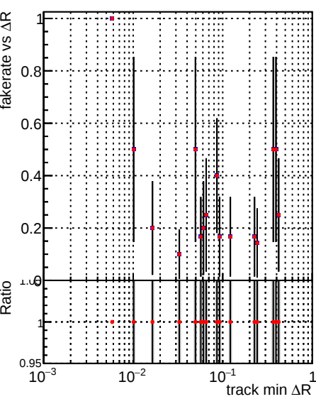
Legend: DQM_CKF_TTbase (grey line with error bars), DQM_CKF_TTtest125xNEW (red dots with error bars)
