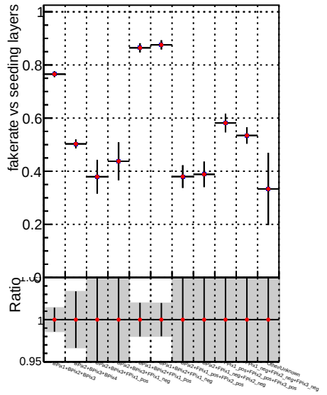
Fake rate vs. DQM_CKF_TTbase DQM_CKF_TTtest125xNEW
