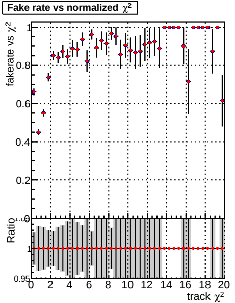
Fake rate vs. DQM_CKF_TTbase DQM_CKF_TTtest125xNEW
