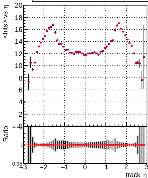
mean hits vs \eta — DQM_CKF_TTbase — DQM_CKF_TTtest125xNEW
