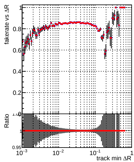
Fake rate vs \Delta R (track, jet) DQM_CKF_TTbase DQM_CKF_TTtest125xNEW
