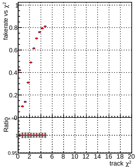
Fake rate vs. —•— DQM_CKF_TTbase —•— DQM_CKF_TTtest125xNEW
