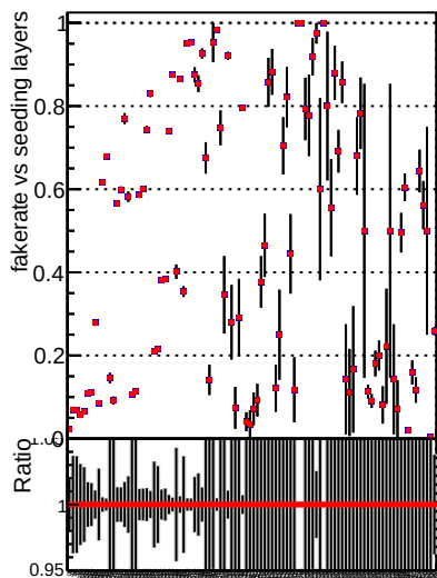
Fake rate vs. —•— DQM_CKF_TTbase —•— DQM_CKF_TTtest125xNEW
