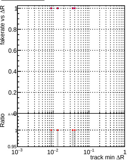
Fake rate vs \Delta R(\text{track, jet}) Legend: \Delta R(\text{track, jet}) (grey line with dots) \Delta R(\text{track, jet}) (red line with dots)
