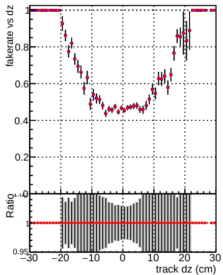
Fake rate vs d —●— DQM_CKF_TTbase —●— DQM_CKF_TTtest125xNEW
