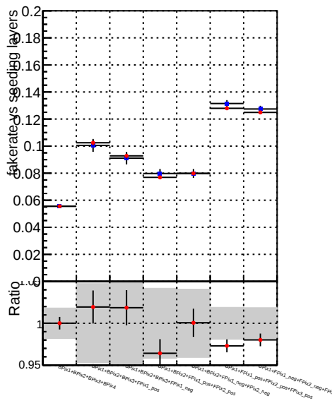
Fake rate vs. Legend: \bullet DQM_mkFit_TTbase, \bullet DQM_mkFit_TTtest125xNEW
