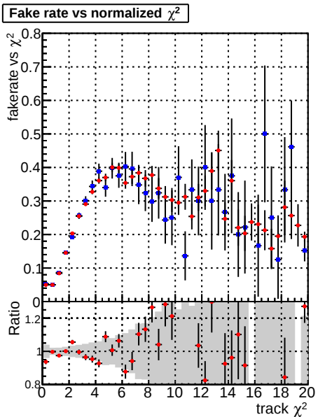
Fake rate vs. Legend: \bullet DQM_mkFit_TTbase, \bullet DQM_mkFit_TTtest125xNEW
