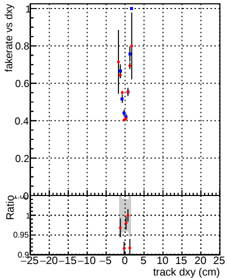
Fake rate vs d — DQM_mkFit_TTbase — DQM_mkFit_TTtest125xNEW
