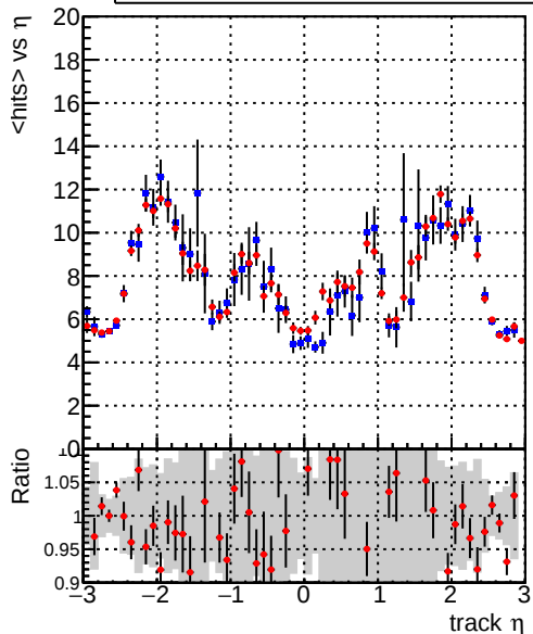
— DQM_mkFit_TTbase — DQM_mkFit_TTtest125xNEW
