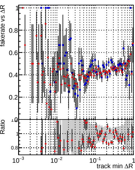
Legend: ■ DQM_mkFit_TTbase ■ DQM_mkFit_TTtest125xNEW
