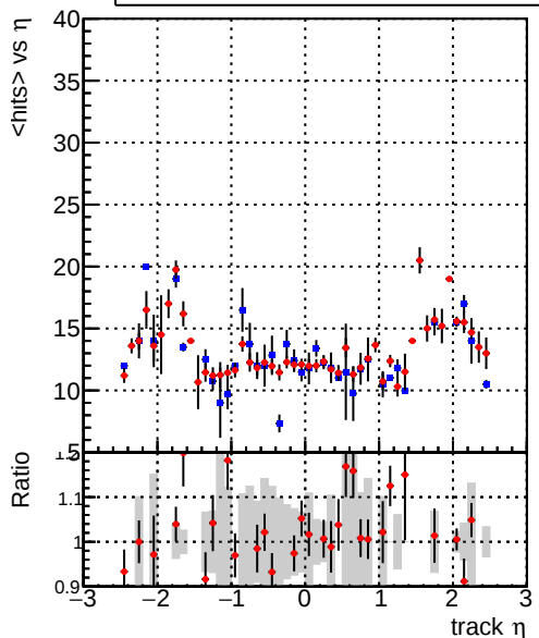
mean hits Legend: DQM_mkFit_TTbase (blue line), DQM_mkFit_TTtest125xNEW (red line)
