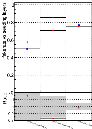
Fake rate vs. — DQM_mkFit_TTbase — DQM_mkFit_TTtest125xNEW
