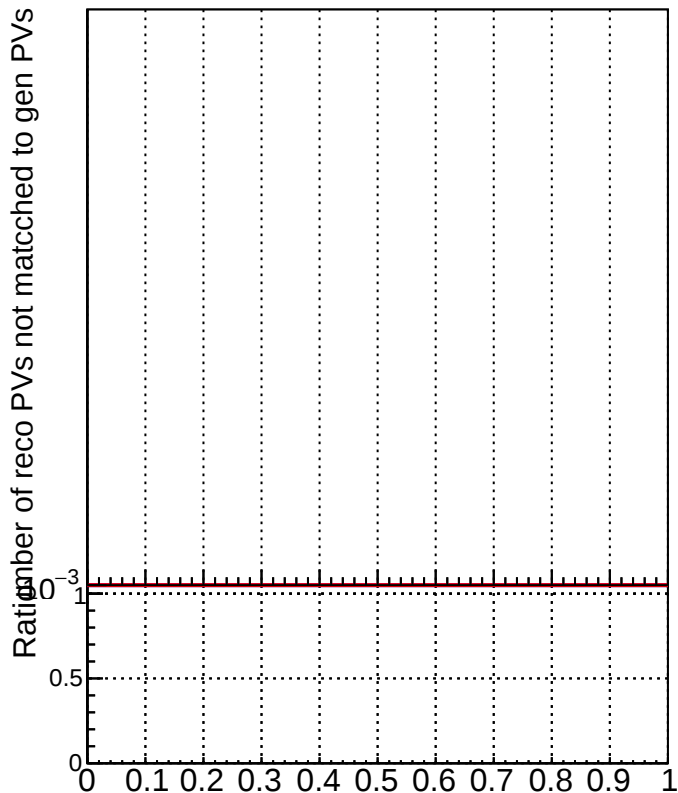
RecoPVAssoc2GenPVnotmatched_missing
